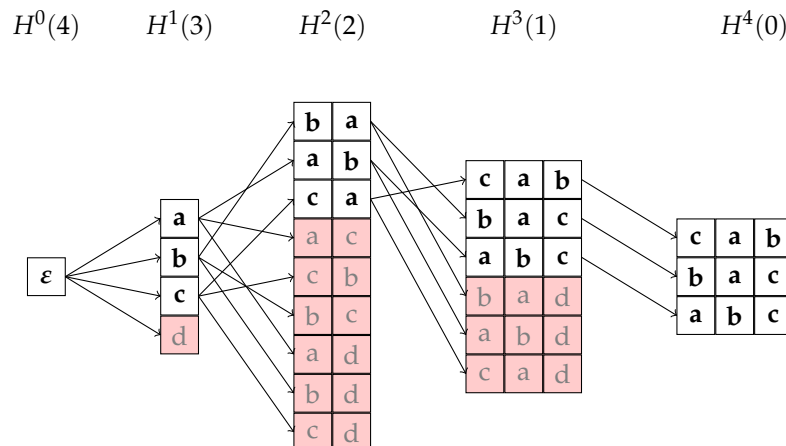
Figure 1: An illustration of the greedy bias in grid beam search with beam width 3. Consider the following setting: There are four constraint tokens: a, b, c, and d. Unigram probabilities are ordered p(a) > p(b) > p(c) > p(d) , but strings starting with low-frequency tokens are slightly more probable than those starting with high-frequency tokens. Assuming no non-constraint tokens, our highest-probability string should be “dcba.” As grid beam search discards early hypotheses with low-frequency constraint tokens, it fails to find this global optimum, and prefers hypotheses which save the hardest constraint ‘d’ for last. For clarity, we only illustrate the generation of constraint tokens, not non-constraint tokens. This results in a depiction of a “diagonal slice” of the grid of beams, where time step and beam depth vary together.
